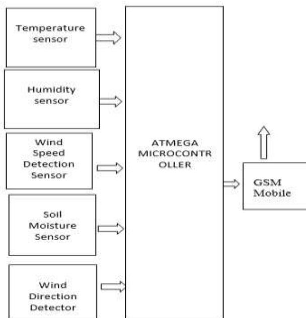
Fig.1 Basic block diagram of proposed system
